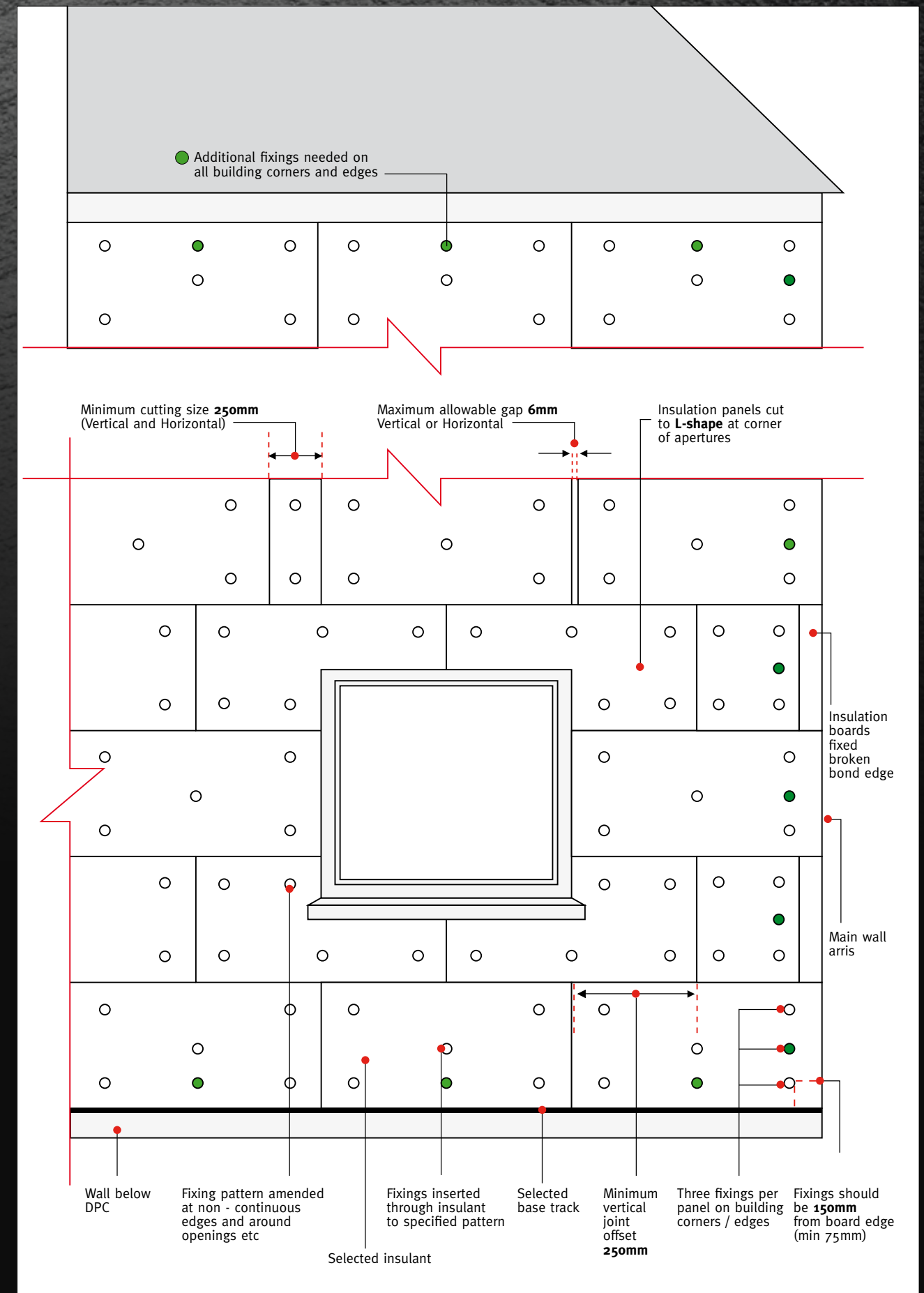
■ Insulation panel pattern guide
