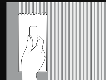
■ Use a notched trowel to create vertical lines in the basecoat prior to the application
