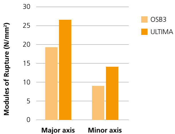
FIGURE 1: 30% increase in mechanical resistance compared to OSB
