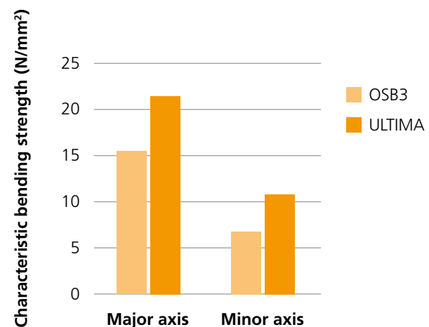
FIGURE 2: 35% increase in characteristic bending strength compared to OSB
