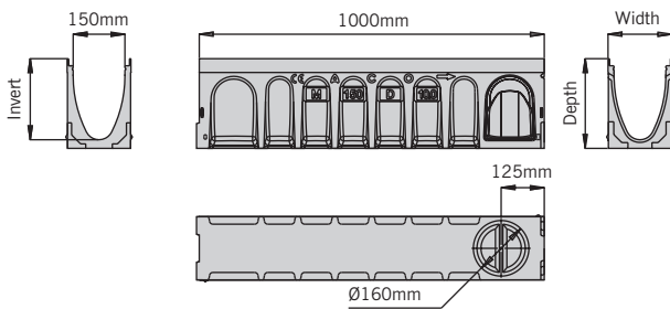
M150D 1m constant depth channel
