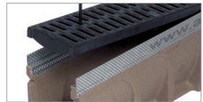
Pull upwards to unlock grating
