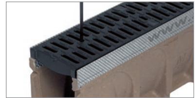
Insert tool as shown. Drainlock™ lifting tool available part no 1367
