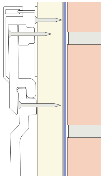
two-part top edge trims — horizontal installation
