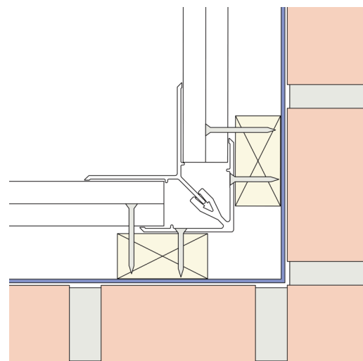
internal corner — horizontal installation
