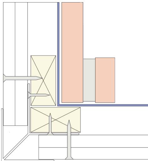
external corner — horizontal cladding
