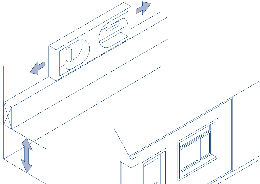
Fig. 1 Check height, line and level of starter batten (Omitt where ventilation is required)
