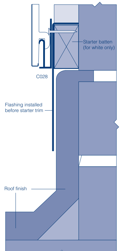
Fig. 7 Wall starter trim C028 above flat roof
