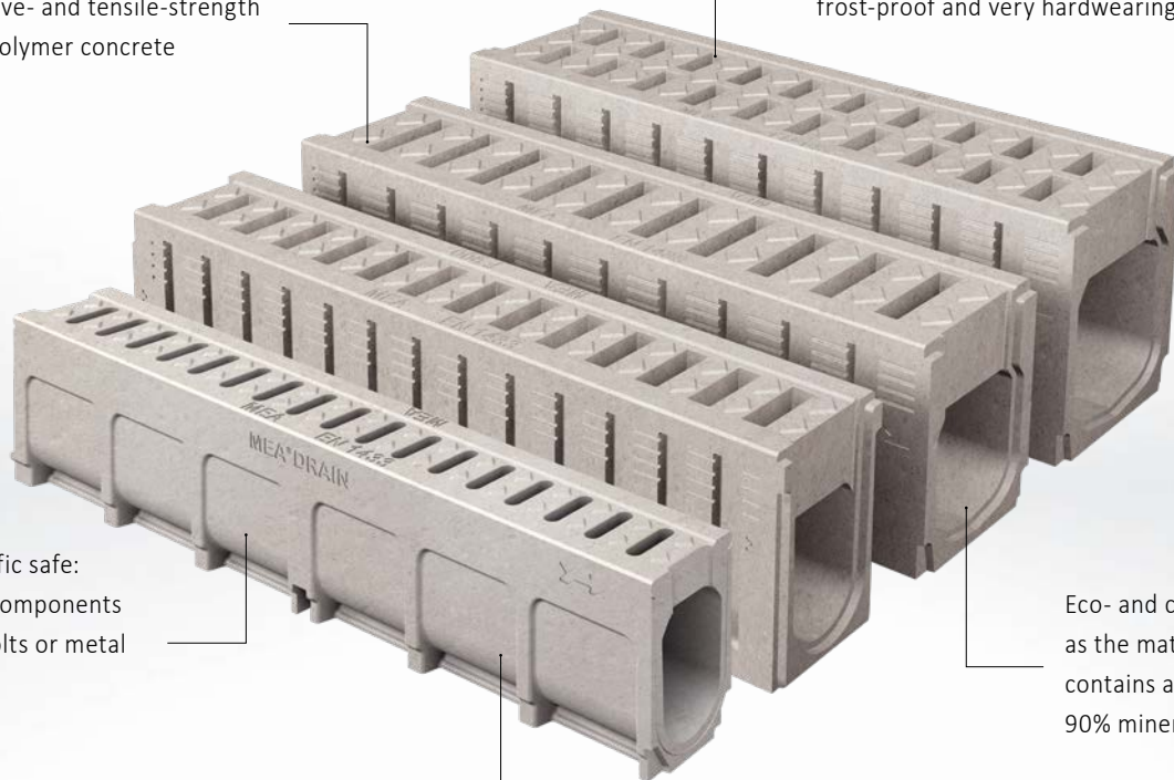
MEADRAIN DM CITY 1000 Loading class up to D 400**
