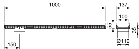
Flat channel MEARIN PLUS F 100, Length: 1 m, construction height: 55 mm
