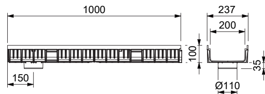
Flat channel MEARIN PLUS F 200, Length: 1 m, Construction height: 100 mm
