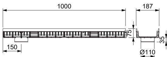
Flat channel MEARIN PLUS F 150, Length: 1 m, Construction height: 75 mm
