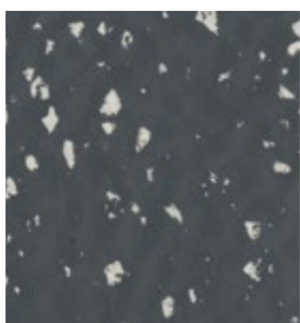
S 14
