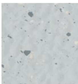
S 104
