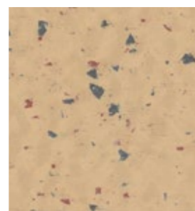
S 17
