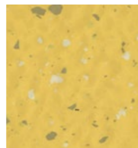
S 106
