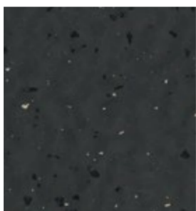
S 32
