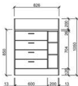
Design with 4 drawers and 3 shelves. Outside width: 826 mm
