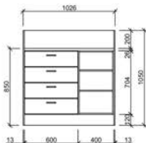
Design with 4 drawers and 3 shelves. Outside width: 1026 mm
