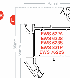
Intermediate transom Z EWS 7023
