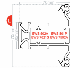
Transom T EWS 7002
