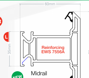
Midrail EWS 7056
