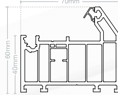
Main frame EWS 7011
