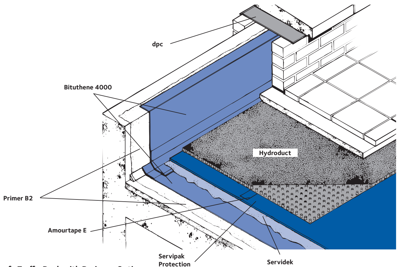
Servirufe Traffic Deck with Drainage Option
