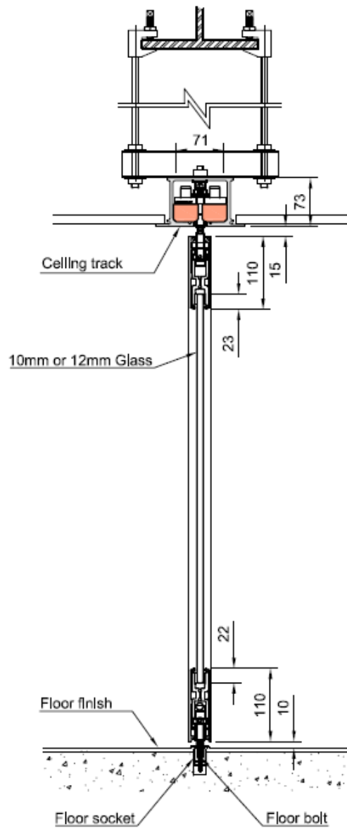
VERTICAL SECTION OF PANEL & TRACK FIXING
