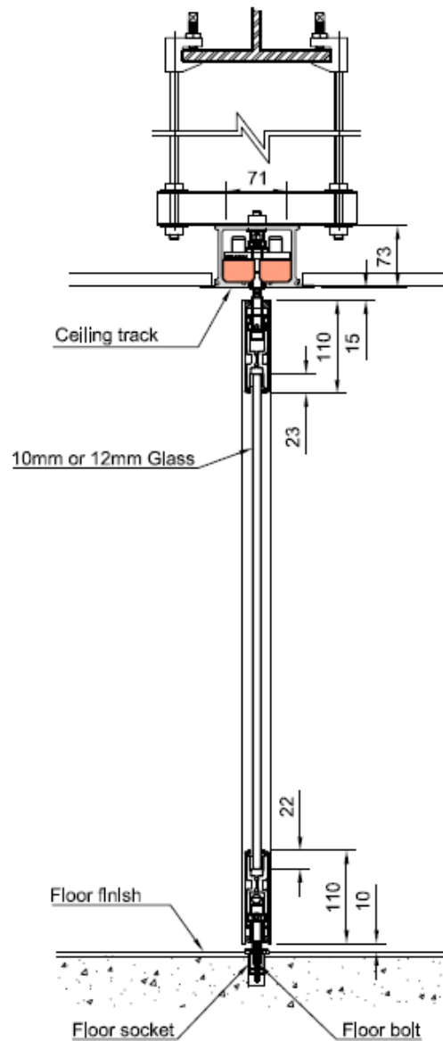
VERTICAL SECTION OF PANEL & TRACK FIXING
