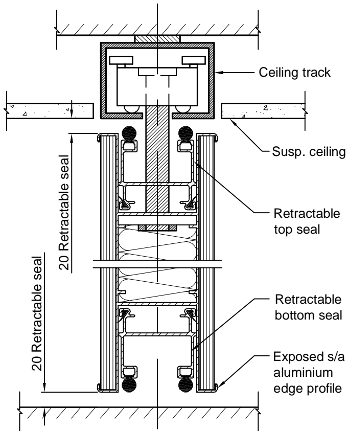
1. VERTICAL SECTION THROUGH STANDARD PANEL
