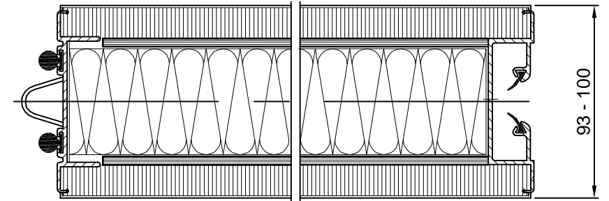
b) Concealed edge profile
