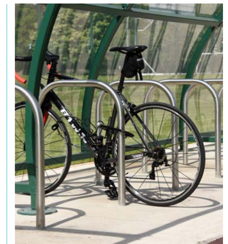
Sheffield Cycle Stand BXMW/GS/SHEFFIELD-STAND
