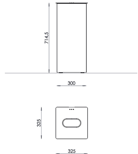
Dimensions (version with feet): H=714,5 mm, L=325 mm, D=300 mm Litter bin capacity: 60 lt Weight: approx. 9 kg
