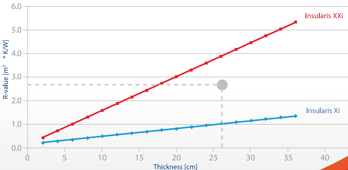
Material performance: Thermal performance as a function of the wall thickness
