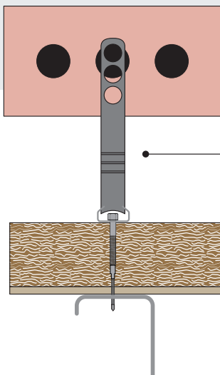
Brick tie channel
