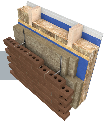
TIMBER FRAME DOUBLE LAYER
